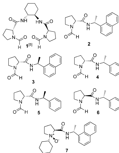
Figure 1. Structures of C 2 -chiral bisformamide 1 , monoformamides 2–6 and proline-derived N -oxide 7 .
